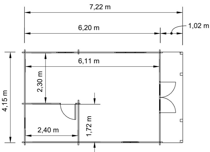
Bottenplan
