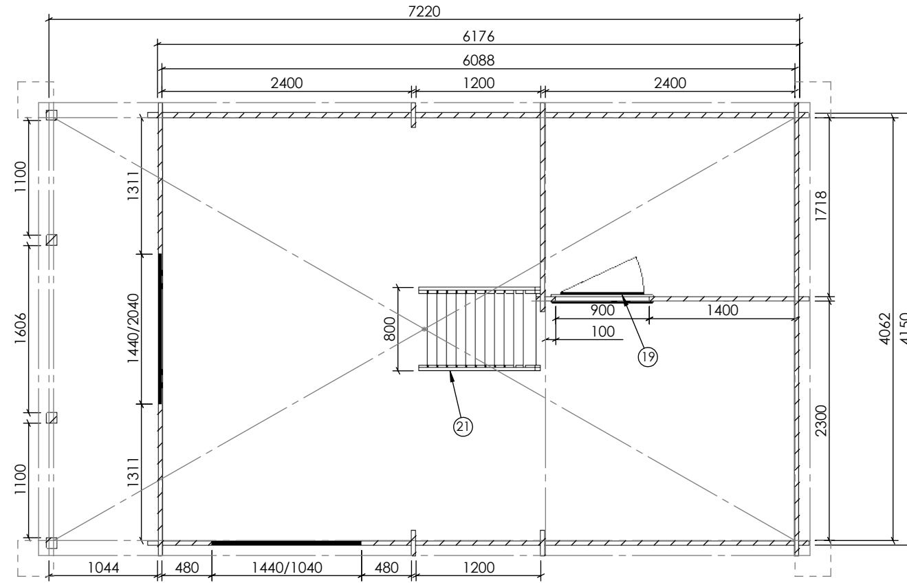
Plan
