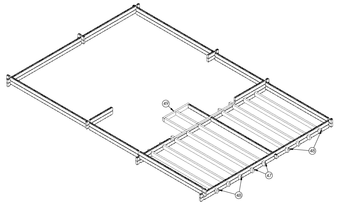
Floor beams 60x140
