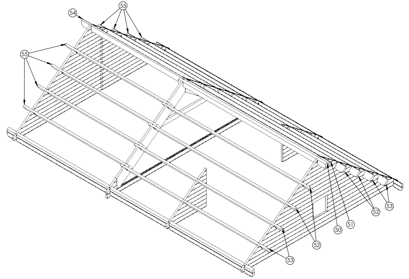
Roof rafters 60x200
