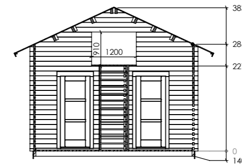
SECTION P-P
