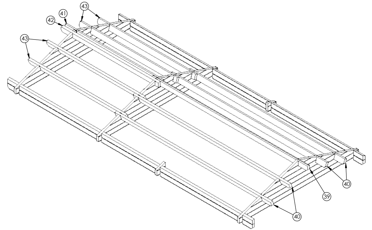
Rafters 60x140
