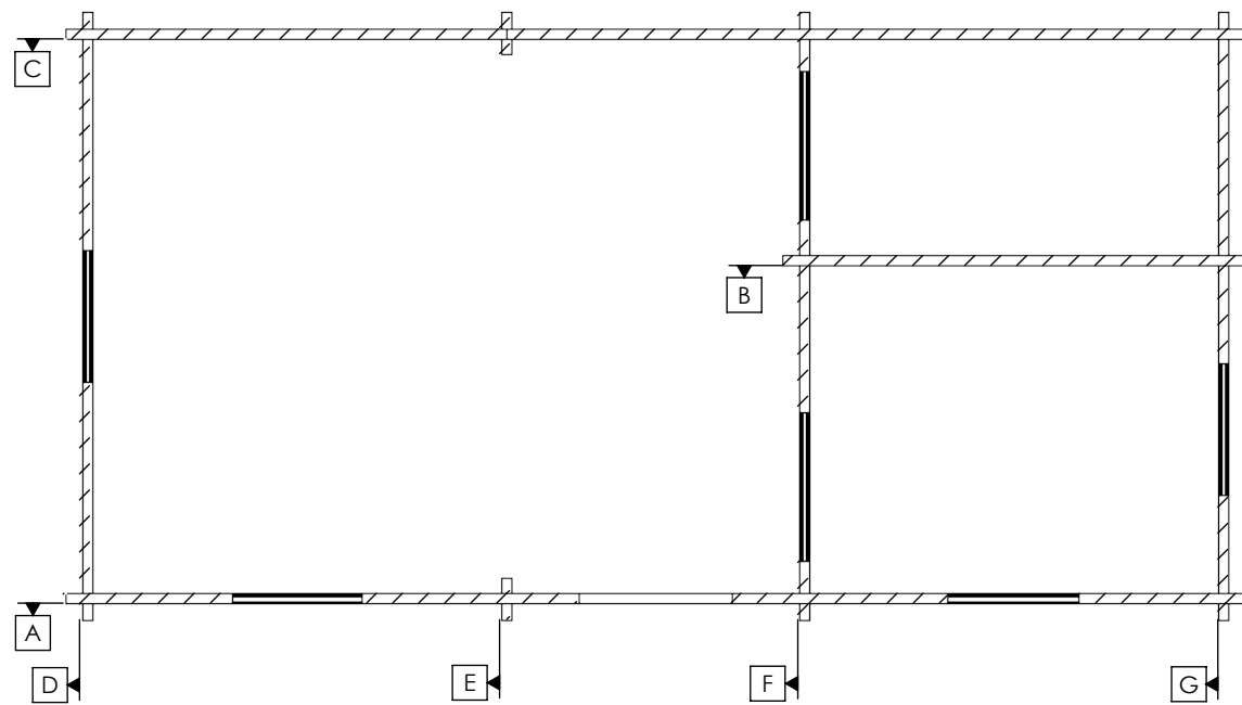
Walls plan
