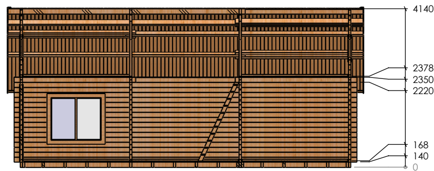
SECTION 1-4 M1:100
