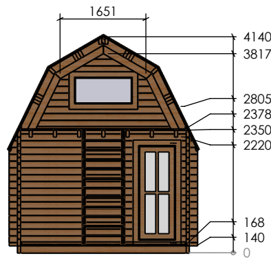
SECTION 3-3 M1:100
