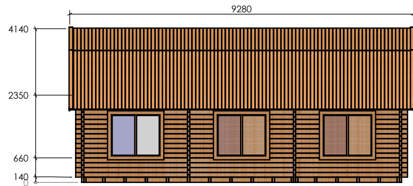
Facade 1-4 M1:100
